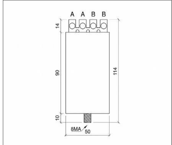
Ignitor DI20 Dimensions
