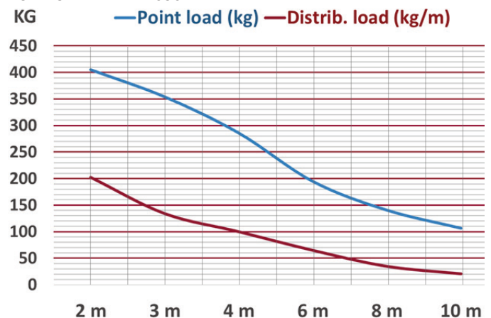
LOAD CHART - EN-1090
