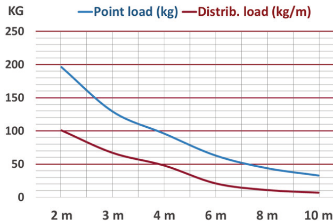
LOAD CHART - EN-1090
